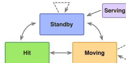
Fig. 1. Proposed four-state-transition behavior model for tennis players.
